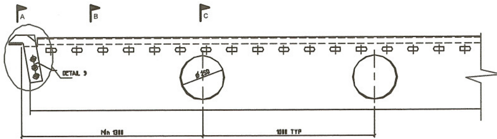
ELEVATION 400 SERIES 16
