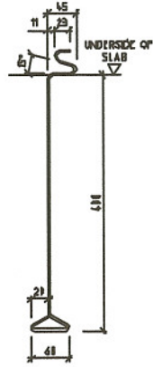
SECTION B-B 16
