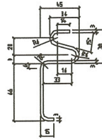
DETAIL 1
