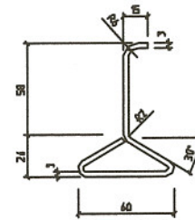
DETAIL 2
