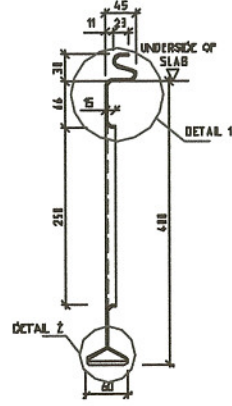
SECTION C-C 16
