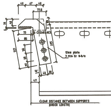
DETAIL 3 15
